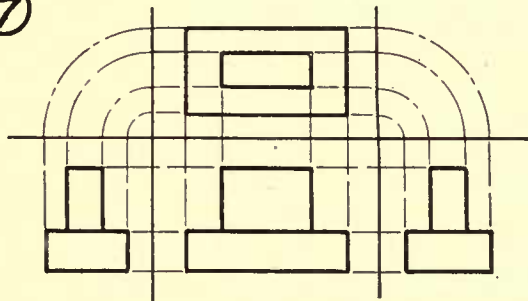
VIEWS OBTAINED BY PROJECTION.
